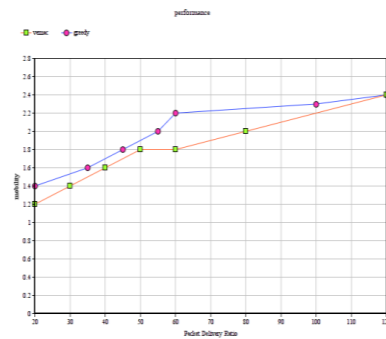
Fig 2: Packet Delivery Ratio vs. mobility
