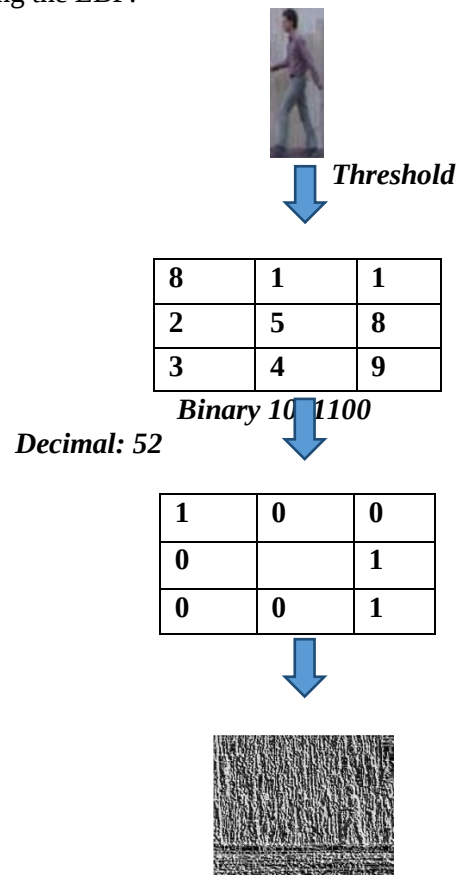
Fig. 6 Feature extraction using the Local Binary Pattern
