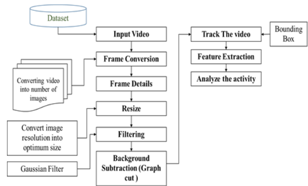
Fig.1. Overall flow of the proposed human activity analysis framework
