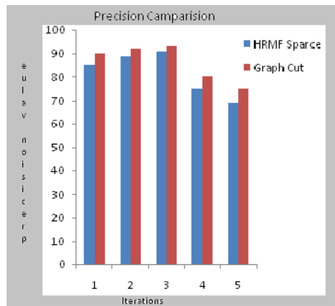
Fig. 9 Comparison of Precision Value for the existing and the proposed segmentation techniques
