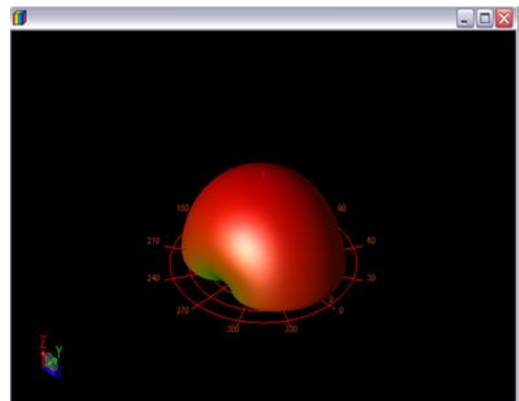
Figure 5. 2 radiation pattern obtained at 854.6 MHz
