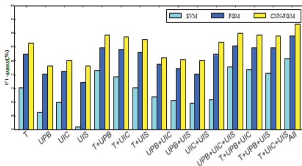
Figure 5. Experiment results analysis of different attribute combinations on different models, with T, UPB, UIC, and UIS
