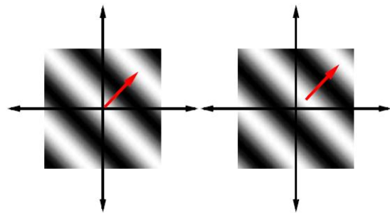
Fig4: The real and imaginary parts of a complex sinusoidal. The images are 128 X128 pixels. The parameters are: u_0 = v_0 = 1=80 cycles/pixel; P = 0 deg.
