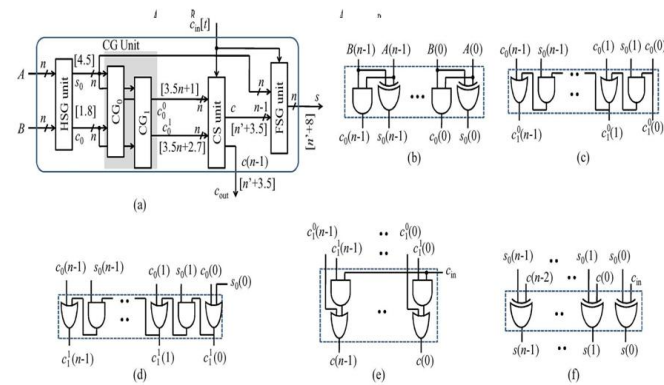
Fig. 3. (a) Proposed CS adder design, where n is the input operand bit-width, and \lceil * \rceil represents delay (in the unit of inverter delay), n = \max(t, 3.5n + 2.7) . (b) Gate-level design of the HSG. (c) Gate-level optimized design of ( CG_0 ) for input-carry = 0. (d) Gate-level optimized design of ( CG_1 ) for input-carry = 1. (e) Gate-level design of the CS unit. (f) Gate-level design of the final-sum generation (FSG) unit.
