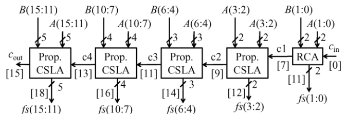
Fig. 4. Proposed SQRD-CSLA for n = 16 . All intermediate and output signals are labeled with delay (shown in square brackets).
