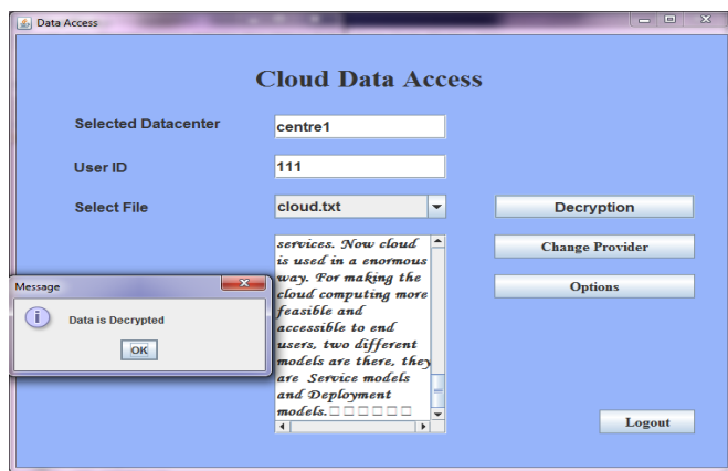
Fig. 9. Decryption process
