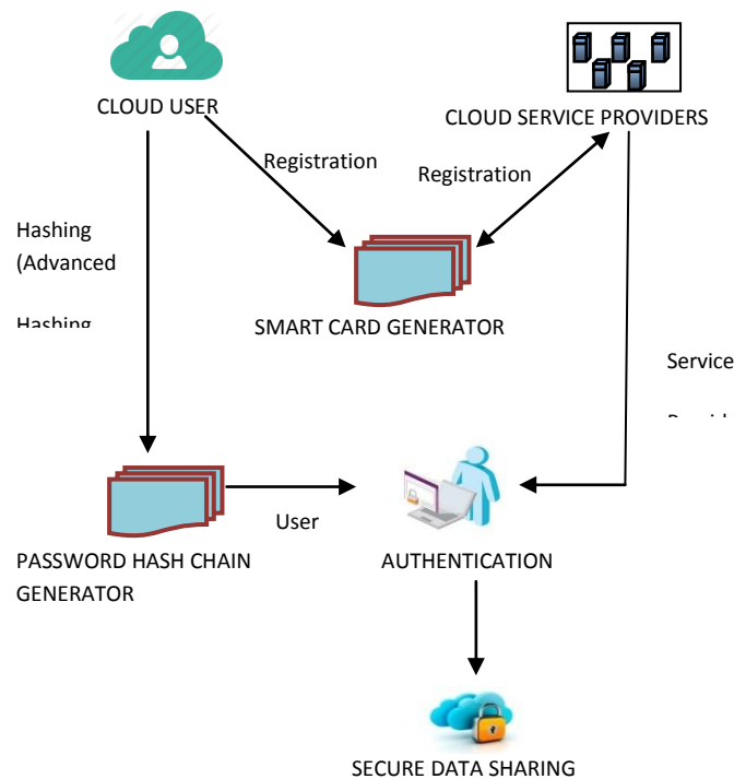
Fig. 5. Authentication scheme-framework.
