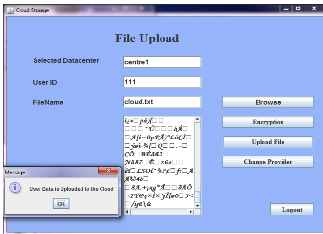
Fig. 8. Encryption process.
