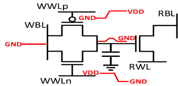
Fig.3. 3T Gain Cell eDRAM
