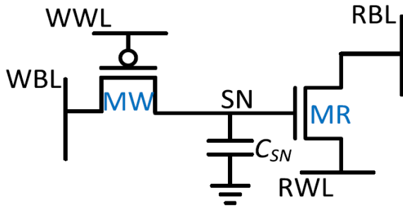
Fig.2. 2T Mixed Gain Cell
