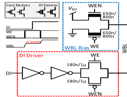
Fig.5. Write Circuitry
